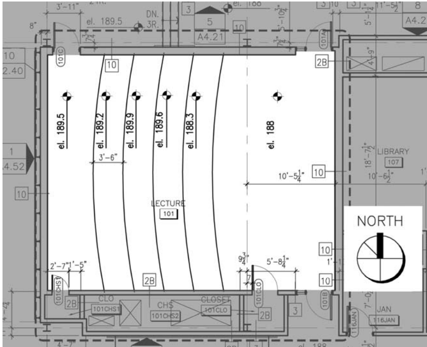
Figure 2: Plan View of Lecture Hall
